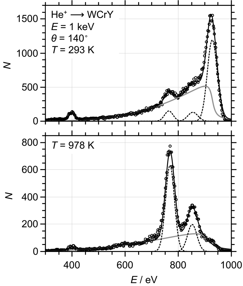
Figure 2: Two LEIS spectra measured at RT (top) and at T = 978 K (bottom). In both spectra the Gaussian peak fits for W, Y, Cr, and O are shown with dotted black lines. The re-ionisation underground is given by the full grey line and the sum of all contributions is plotted with the full black line.
