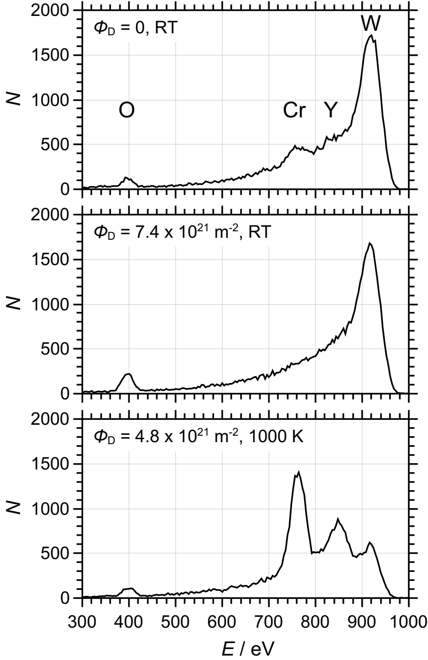
Figure 7: LEIS spectra showing the preferential sputtering of the lighter alloy constituents. The labels indicate the species which cause the respective scattering peaks. The spectrum after sputter cleaning with Kr is plotted at the top. The plot in the middle shows the spectrum after D sputtering with a fluence of 7.4 \times 10^{21} \text{ m}^{-2} at RT. The plot at the bottom displays the spectrum after a D sputter fluence of 4.8 \times 10^{21} \text{ m}^{-2} at a sample temperature of 1000 K.
