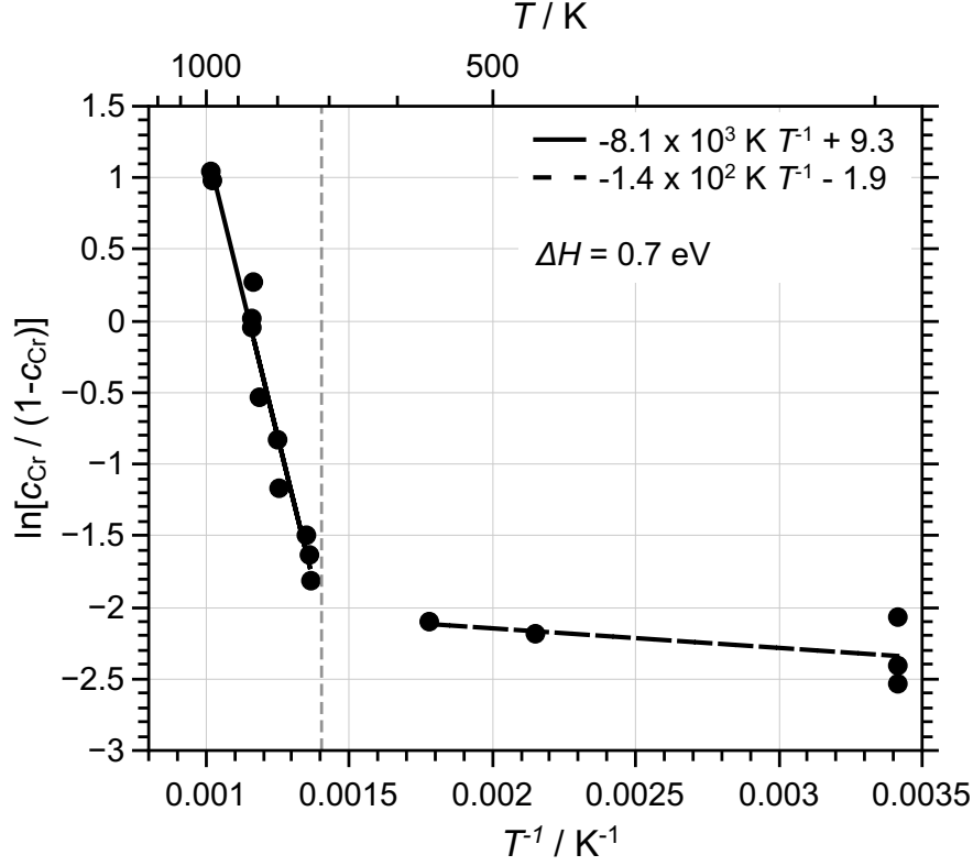
Figure 4: Arrhenius plot of the Langmuir-McLean relation (equation 3) for Cr with straight line fits for the high temperature (above 700 K) and low temperature regions. The logarithm of the surface coverage, \ln(\frac{c_{\text{Cr}}^s}{1 - c_{\text{Cr}}^s}) , is plotted versus the reciprocal temperature, T^{-1} . A temperature scale is drawn on top of the figure.
