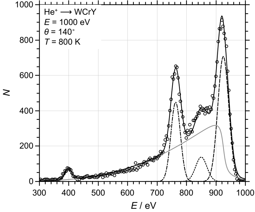
Figure 1: LEIS spectrum measured at a sample temperature of 800 K. The number of counts, N , is plotted versus the energy, E , of the respective channel. Measured data points are drawn with open circles, the peaks in the spectrum are fitted with Gaussians: Cr (dashed-dotted line), Y(dotted line), W(dashed line). The re-ionisation background from W is plotted with the grey line. The small peak at 400 eV originates from O. The sum of all contributions is given by the full black line.
