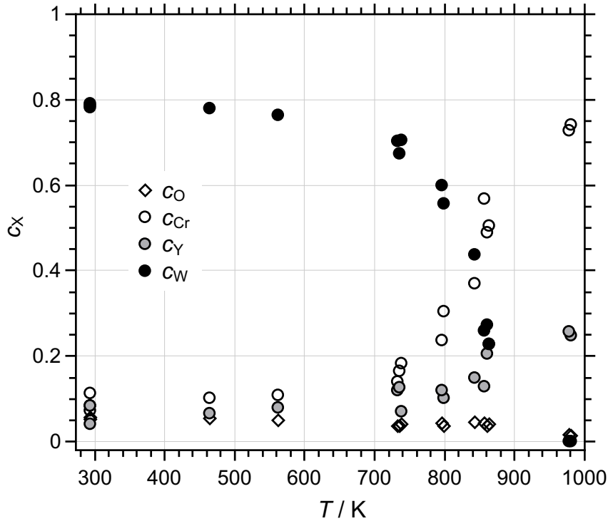
Figure 3: The fractional surface concentrations, c_X , determined from the fitted peaks in the LEIS spectra according to equation 2 for O, Cr, Y, and W are plotted versus the sample temperature, T .
