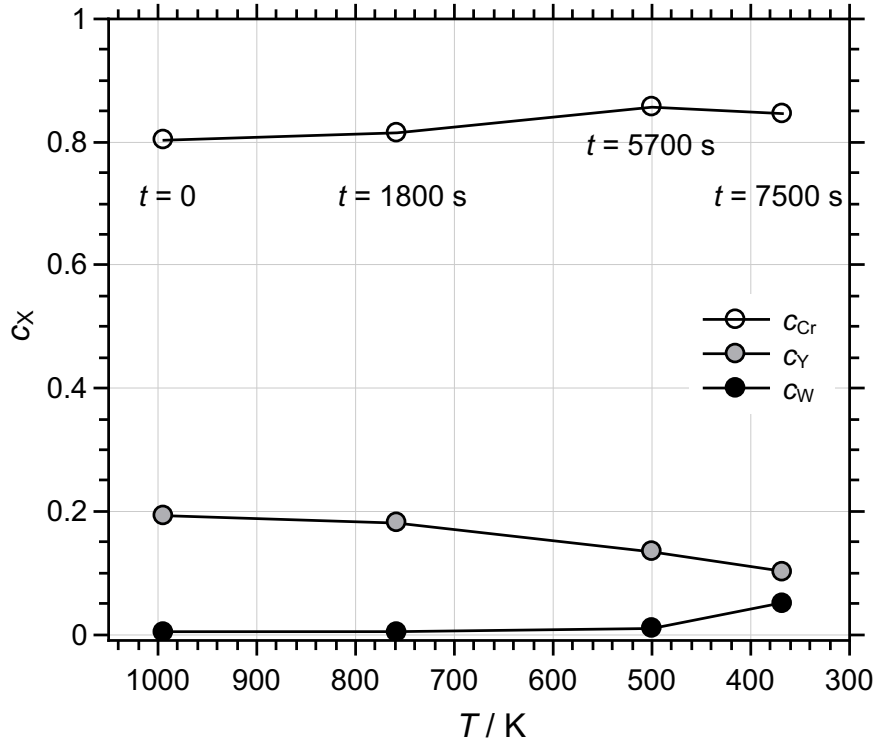
Figure 6: Fractional surface concentrations, c_X , measured for various temperatures during cooling of the sample. The measurements proceed from left to right. Note that the temperature scale, T , is inverted. The times when each spectrum has been measured are indicated in the figure.
