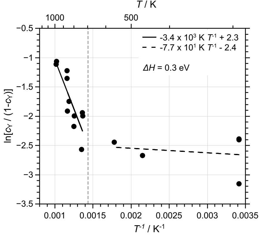
Figure 5: Arrhenius plot of the Langmuir-McLean relation (equation 3) for Y with straight line fits for the high temperature (above 700 K) and low temperature regions. The logarithm of the surface coverage, \ln(\frac{c_Y^s}{1-c_Y^s}) , is plotted versus the reciprocal temperature, T^{-1} .
